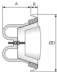
Figure 4. Exhaust register EXC.
