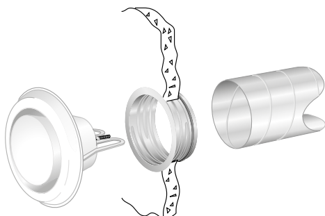
Figure 1. Installation.
